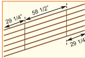
10' panel measurements
