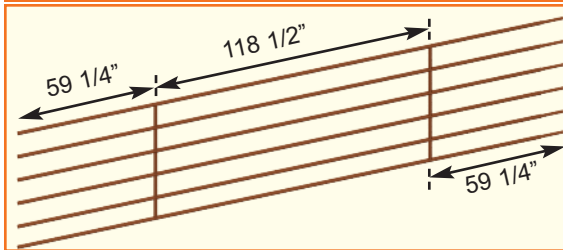
20' panel measurements
